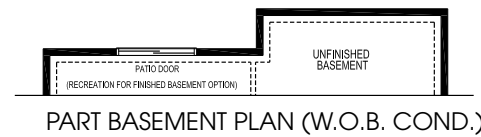
PART BASEMENT PLAN (W.O.B. COND.)
